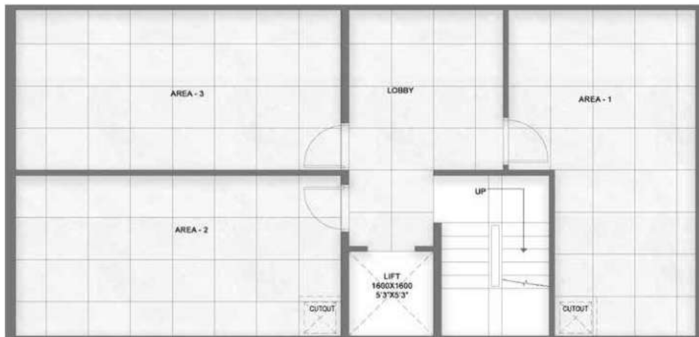
BASEMENT PLAN
